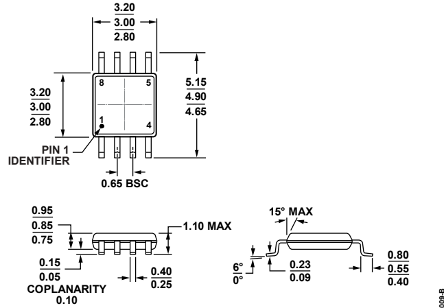
Figure 71. 8-Lead Mini Small Outline Package [MSOP] (RM-8)
