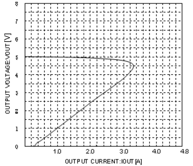
Fig.16 Load Stability
