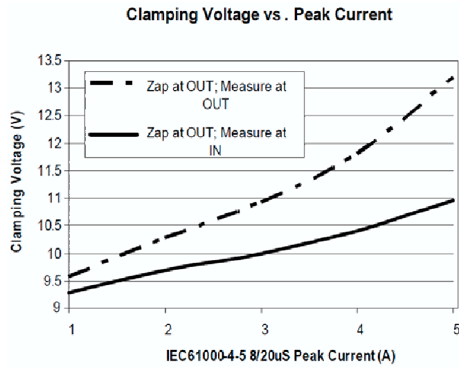
Figure 11. Clamping Voltage vs. Peak Current
