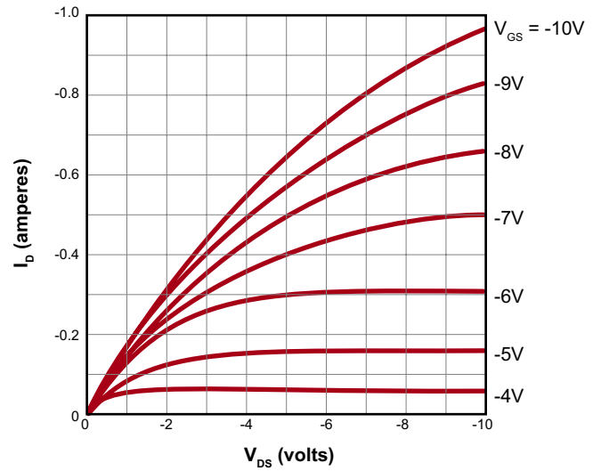
Saturation Characteristics
