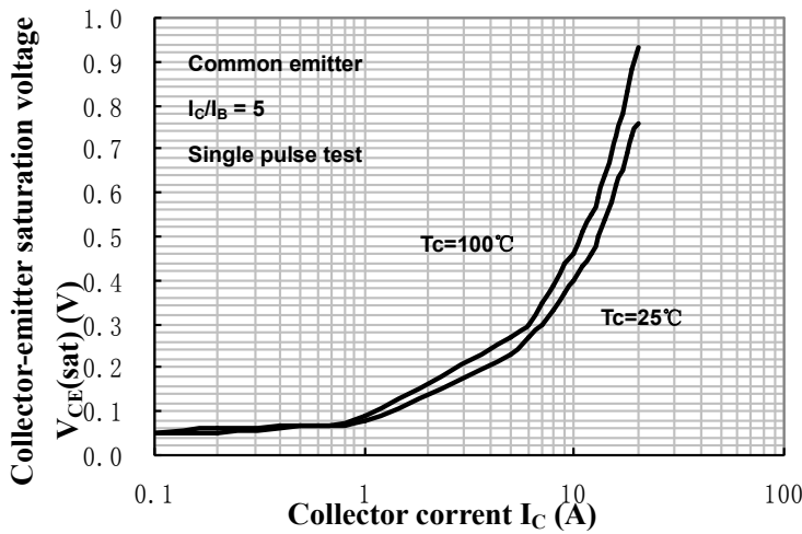
Saturation Voltage
