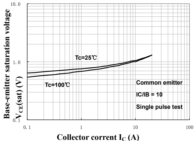
Base-Emitter Voltage
