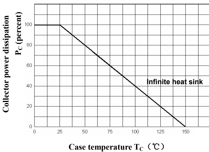
Power Derating
