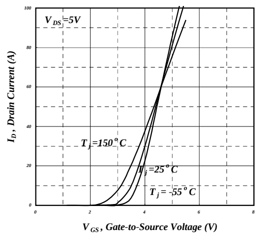
Fig 15. Transfer Characteristics
