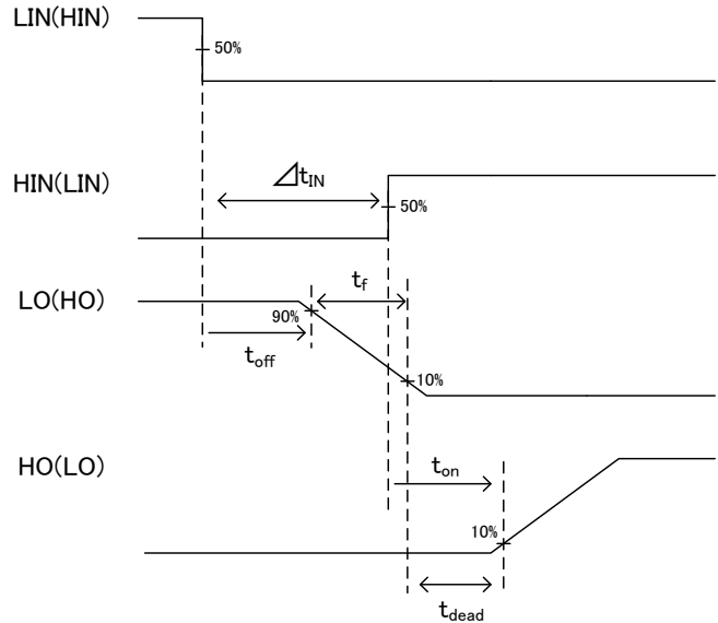
Figure 29. Shoot-Through Prevention Timing Chart
