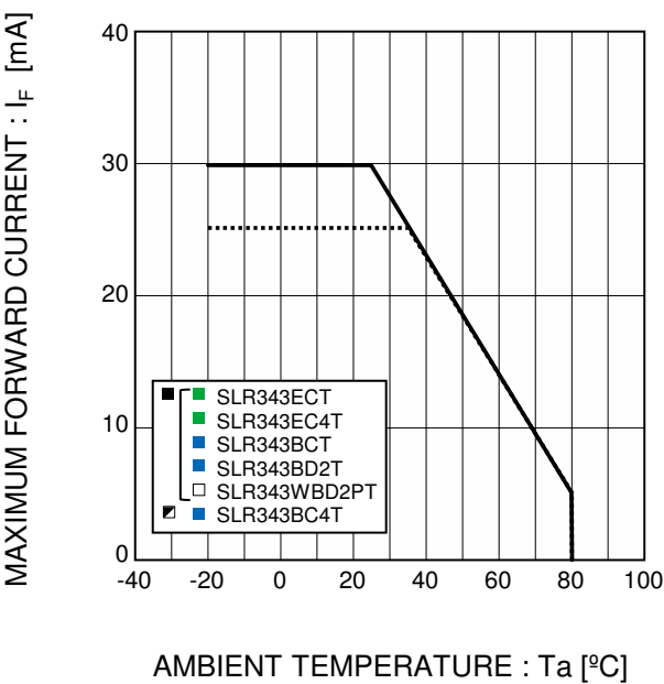
Fig.4 Derating
