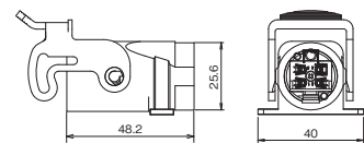
Receptacle Housing
