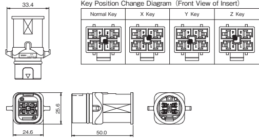
Receptacle Housing
