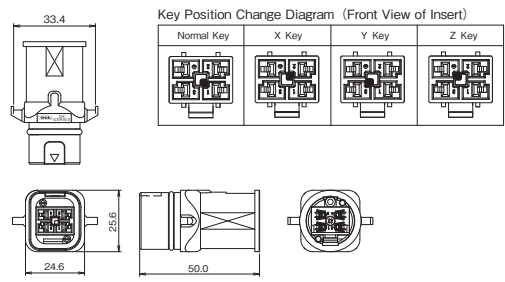
Receptacle Housing
