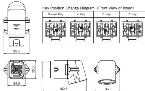
Receptacle Housing
