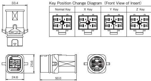
Tab Housing
