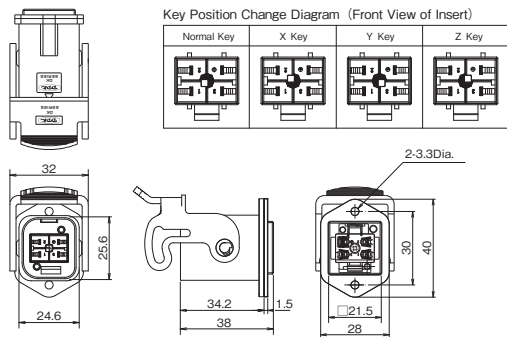
Tab Housing
