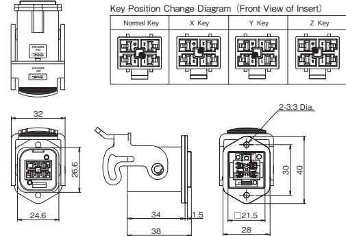
Receptacle Housing
