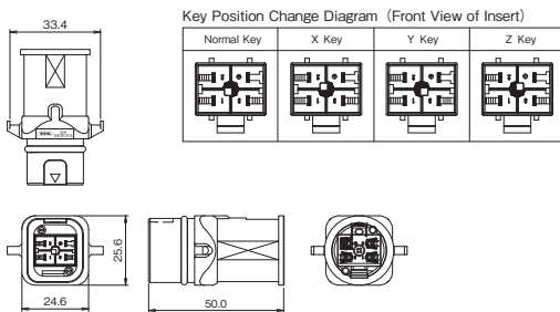
Tab Housing
