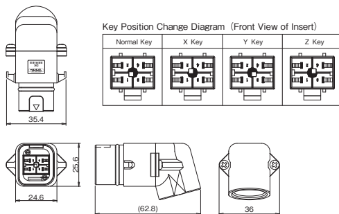
Tab Housing
