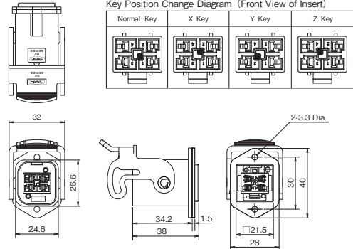
Receptacle Housing
