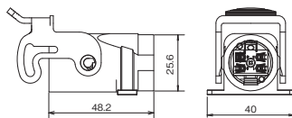
Tab Housing
