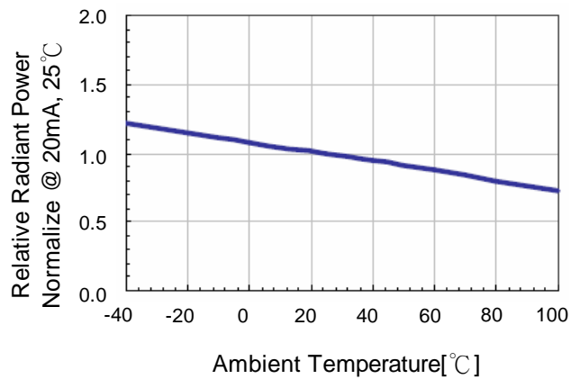
Fig.4 Relative Radiant Power vs. Temperature
