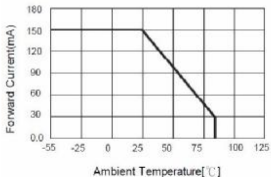
Fig.5 Forward Current vs. Temperature
