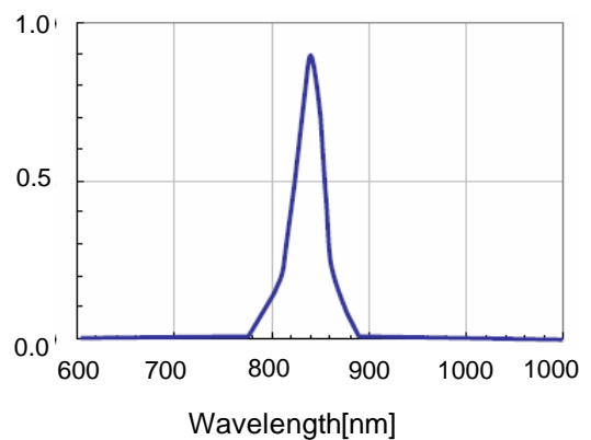
Fig.6 Relative Intensity vs. Wavelength
