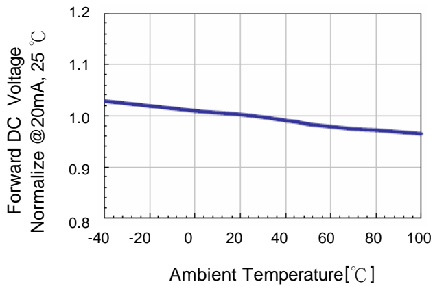
Fig.3 Forward DC Voltage vs. Temperature
