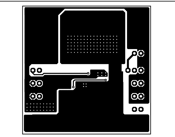
Figure 73: Bottom layer
