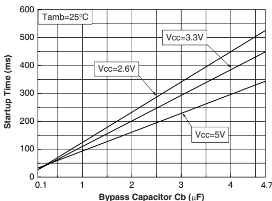
Figure 66: Typical wake-up time vs. C_B
