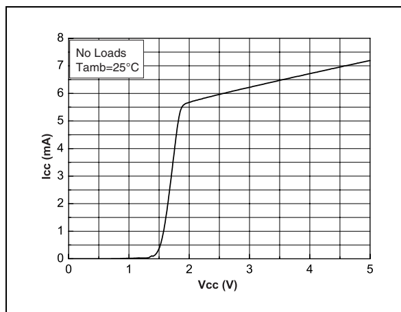
Figure 37: Current consumption vs. standby voltage at Vcc=5V
