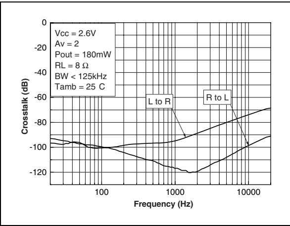
Figure 60: Crosstalk vs. frequency
