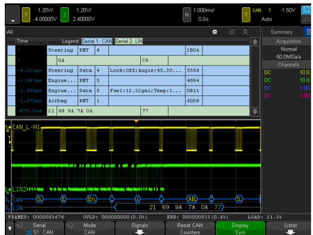
Figure 20. Dual serial bus CAN and LIN decode and interleaved "lister" display.
