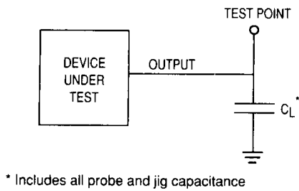
Figure 5. Test Circuit
