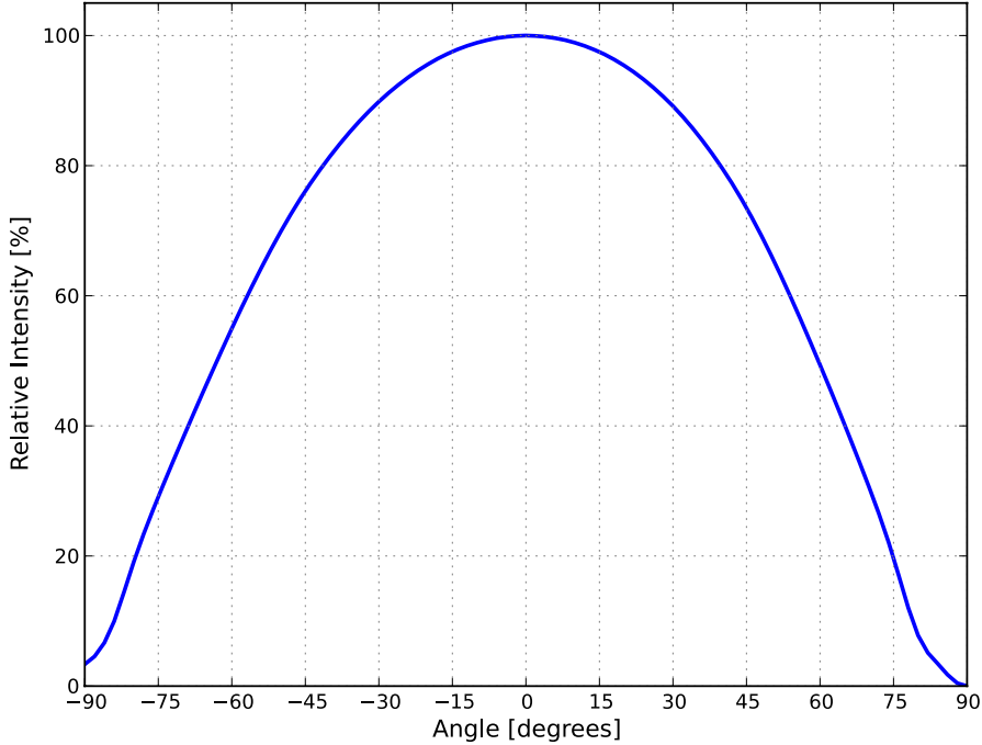
Figure 4a: Typical radiation pattern for LXHx-FWxx at 700mA, T_j=85^\circ\text{C} .
