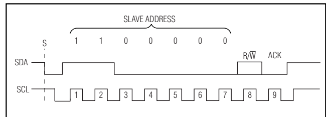
Figure 1. MAX2120 Slave Address Byte
