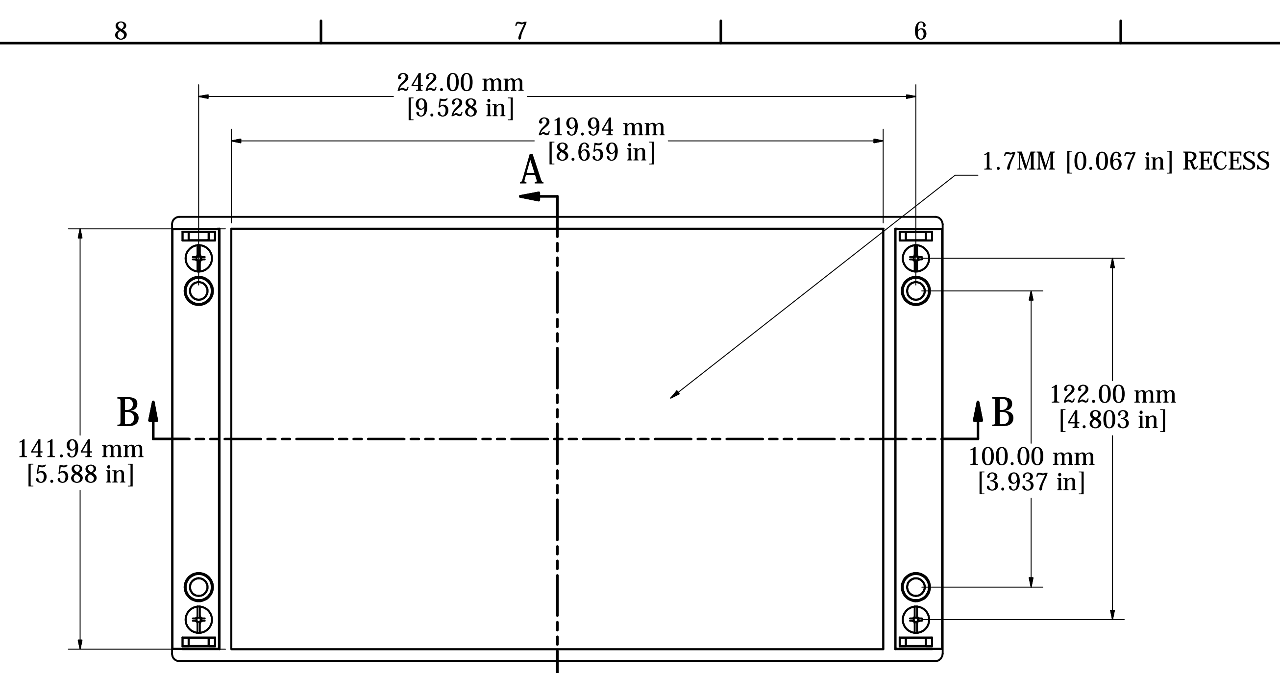
ASSEMBLY - TOP VIEW
