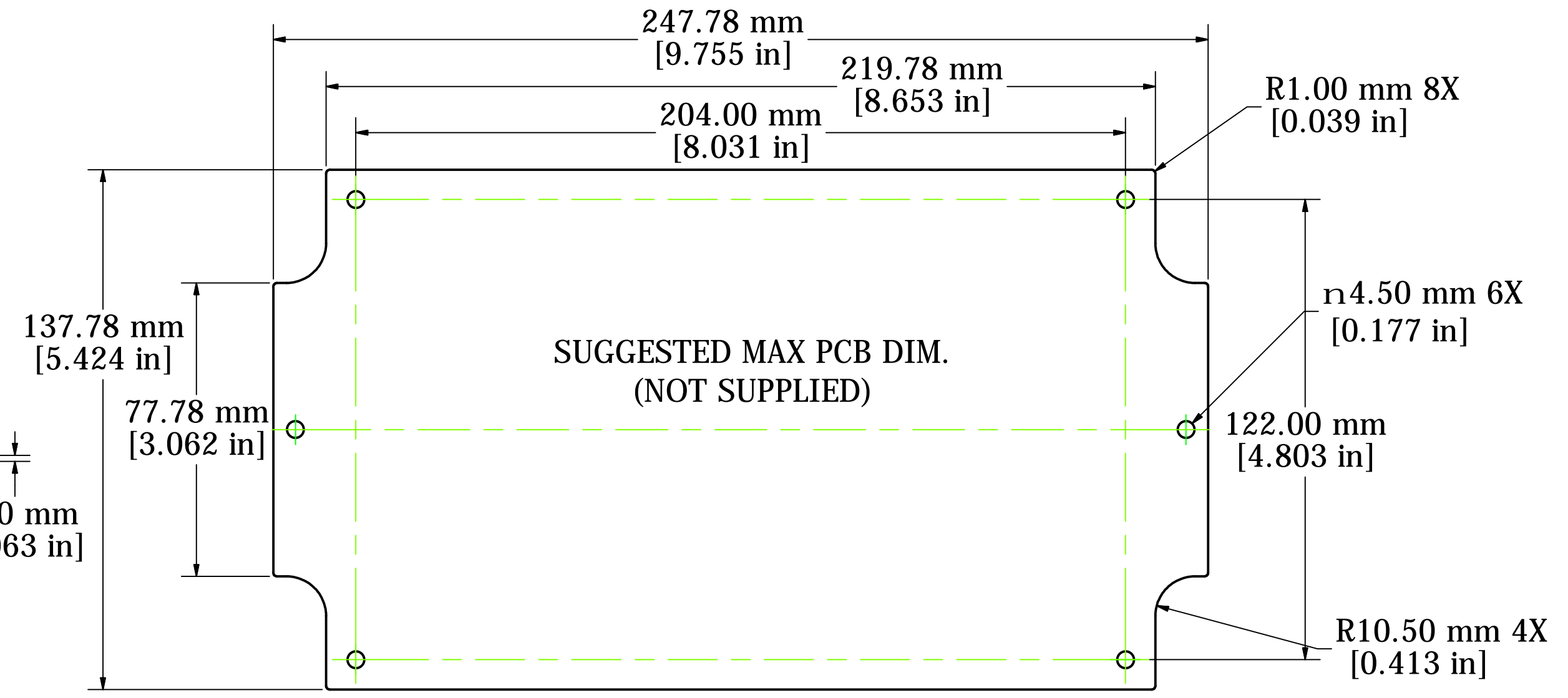
PCB
