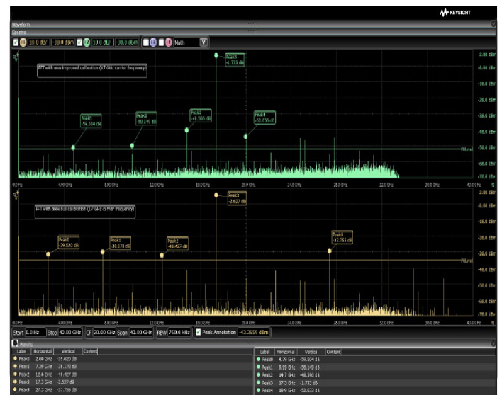
Improved calibration increases the spurious free dynamic range by up to 15 dBc.
