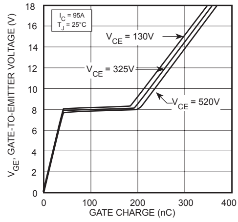
FIGURE 11, Gate charge
