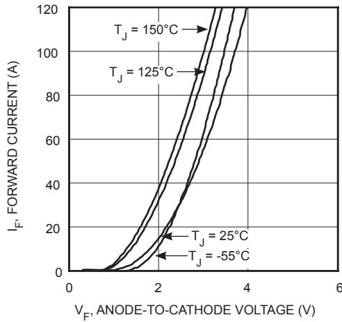
FIGURE 19, F Forward Current vs. Forward Voltage
