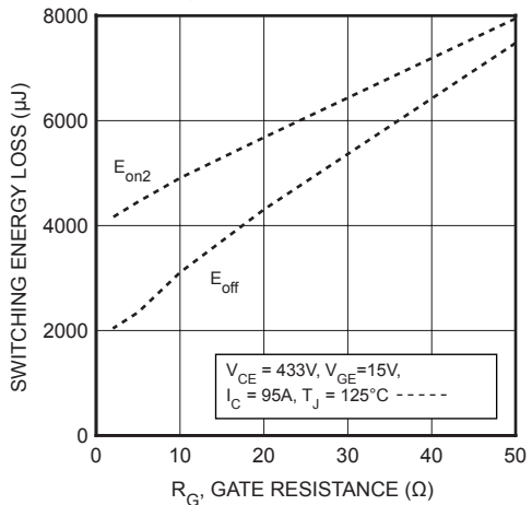
FIGURE 15, Energy Loss vs Gate Resistance
