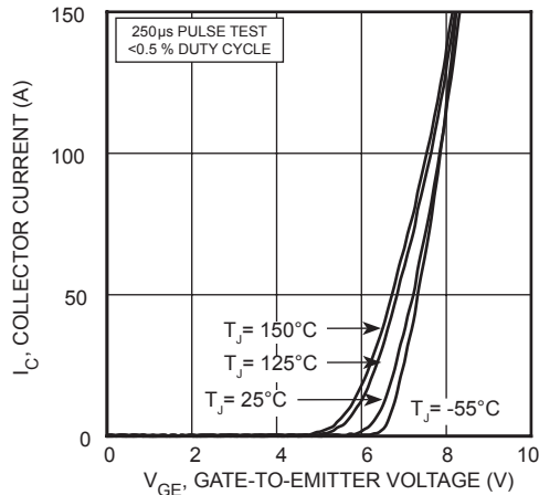
FIGURE 6, Transfer Characteristics
