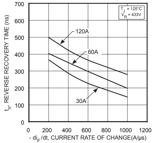
FIGURE 20, Reverse Recovery Time vs. Current Rate of Change
