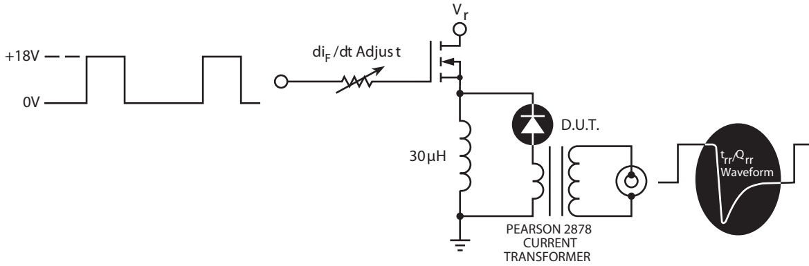
FIGURE 25. Diode Test Circuit
