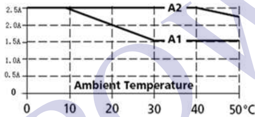
Output Current
