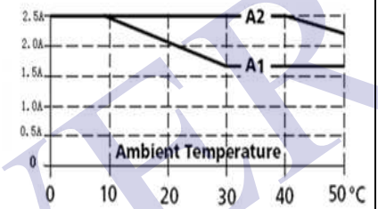
Output Current
