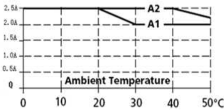
Output Current
