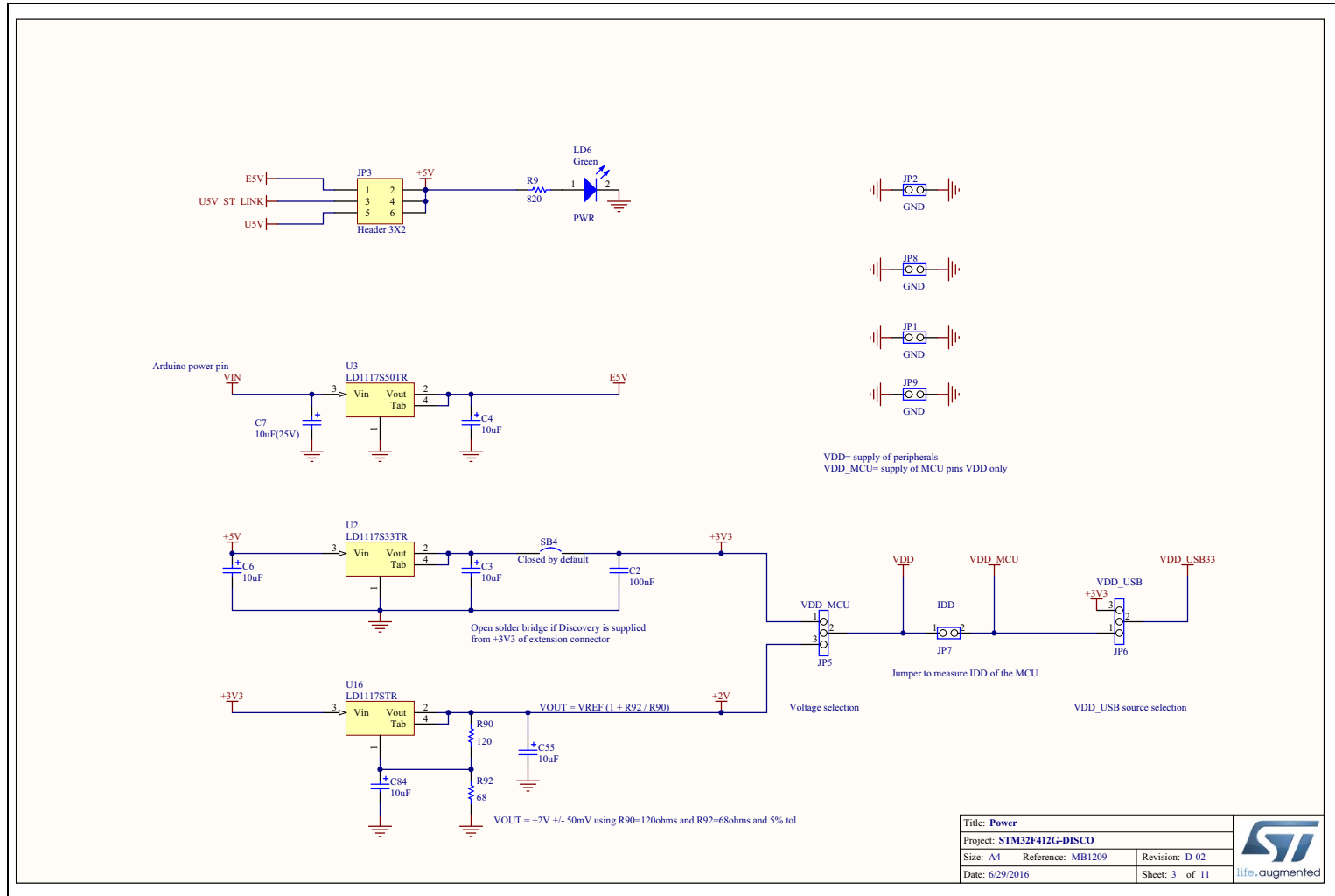
Figure 15. 32F412GDISCOVERY Power
