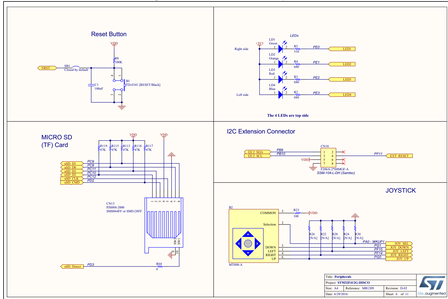
Figure 19. 32F412GDISCOVERY Peripherals
