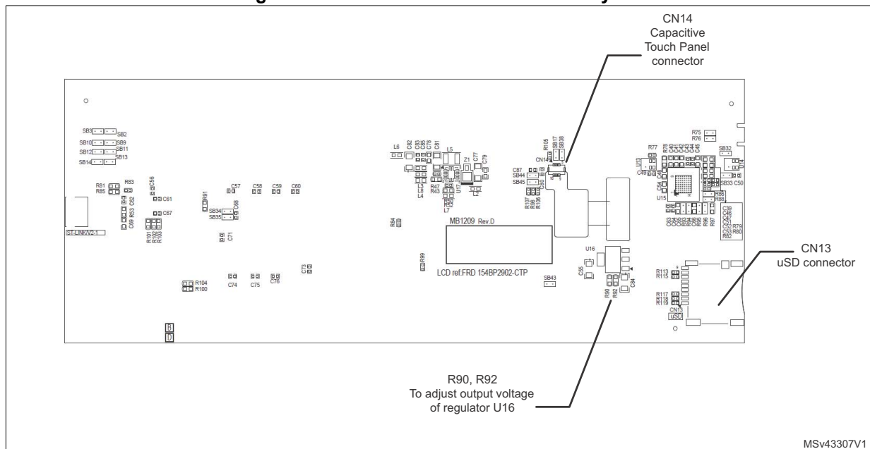
Figure 5. 32F412GDISCOVERY bottom layout
