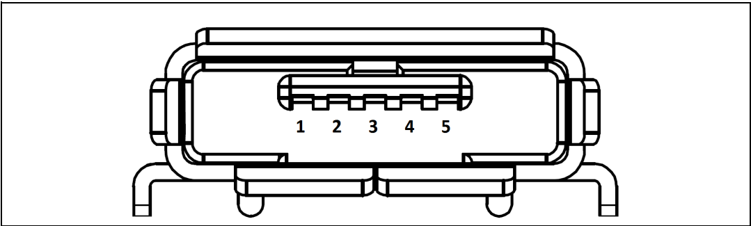
Figure 10. USB OTG FS Micro-AB connector CN3 (front view)
