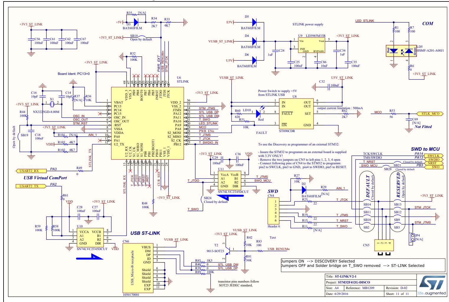
Figure 23. 32F412GDISCOVERY ST-LINK/V2-1
