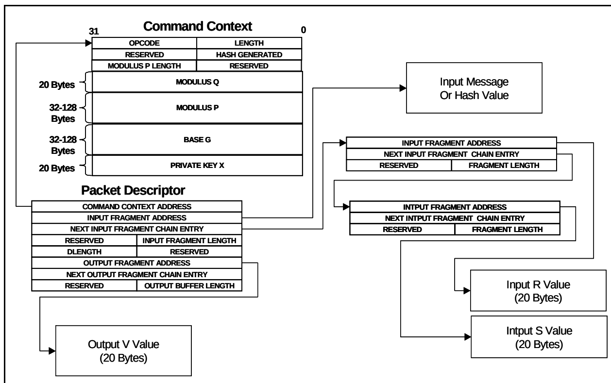
Figure 30: DSA Verify
