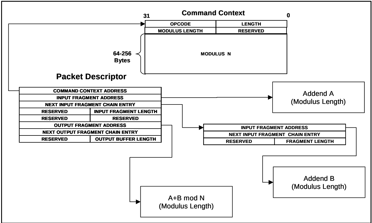
Figure 32: Modular Add
