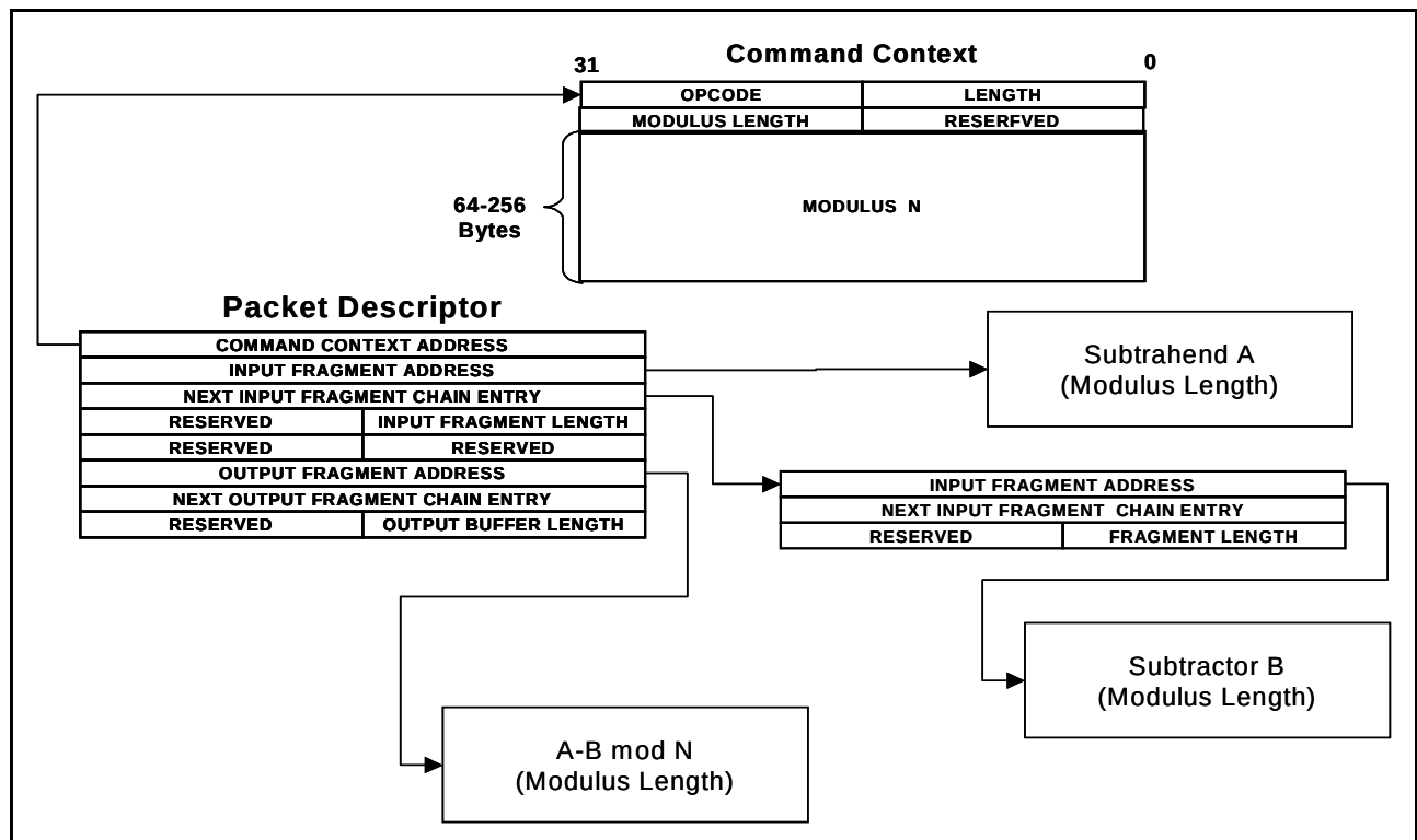
Figure 33: Modular Subtract
