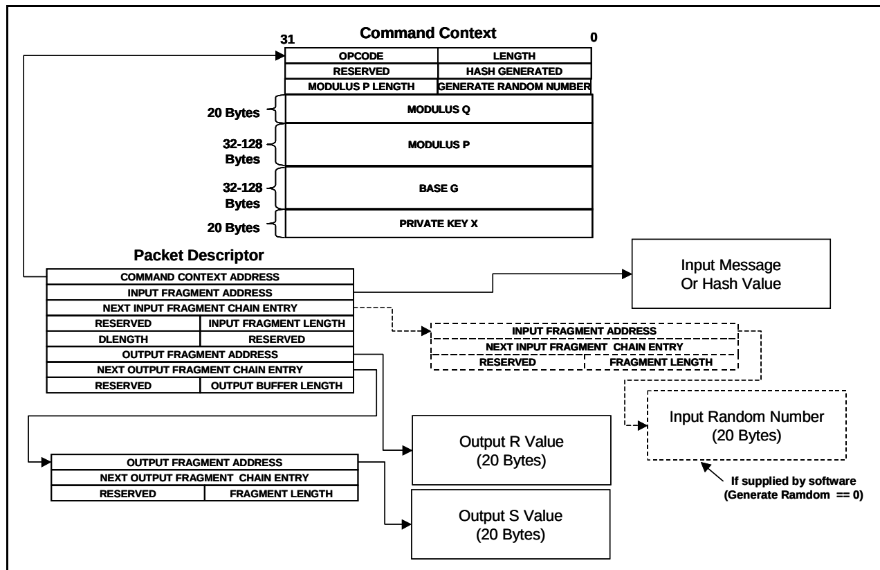
Figure 29: DSA Sign
