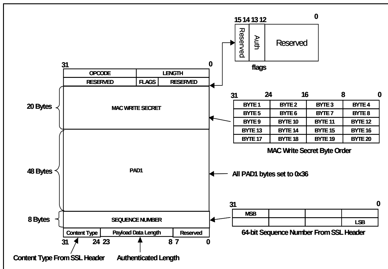
Figure 14: SSL MAC Command Context
