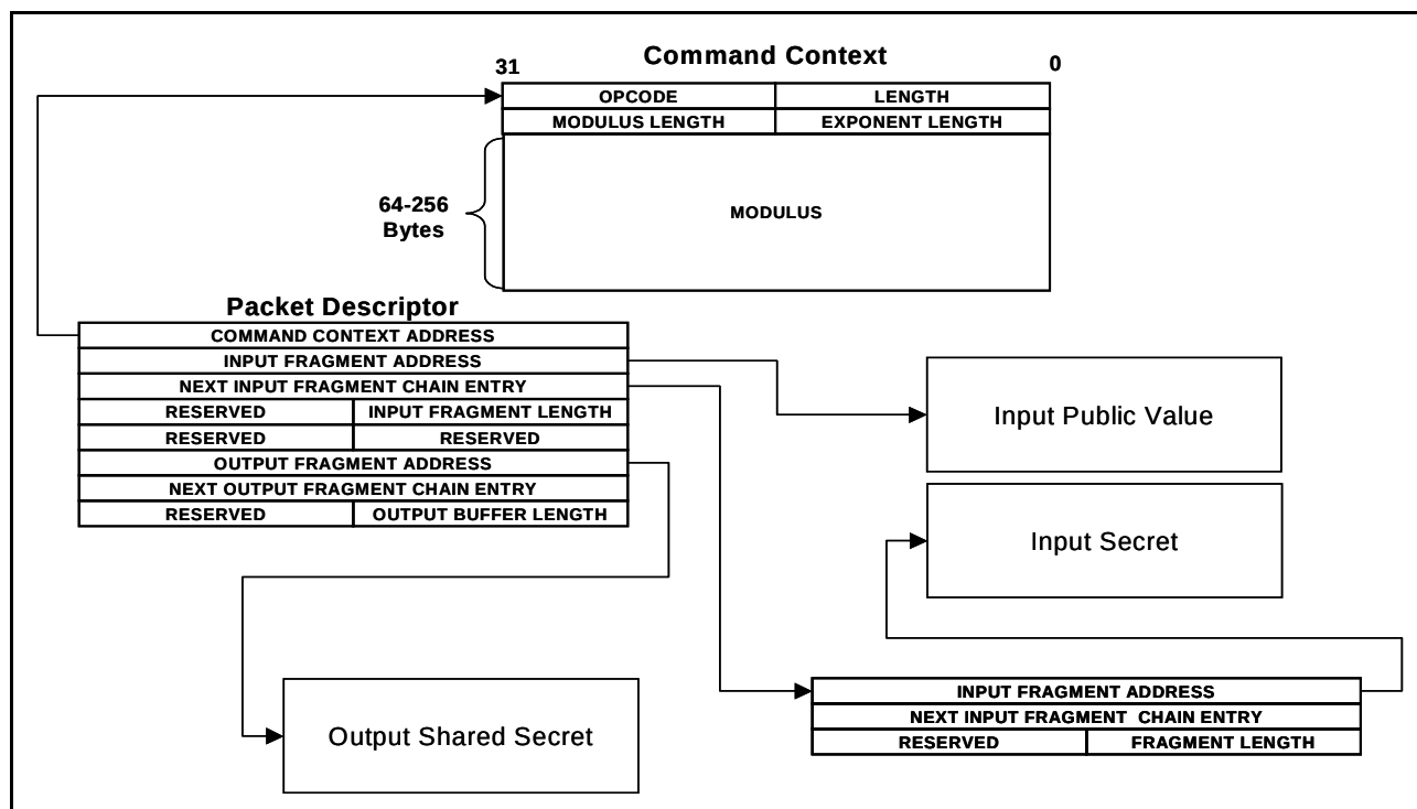
Figure 26: Diffie-Hellman Secret Key
