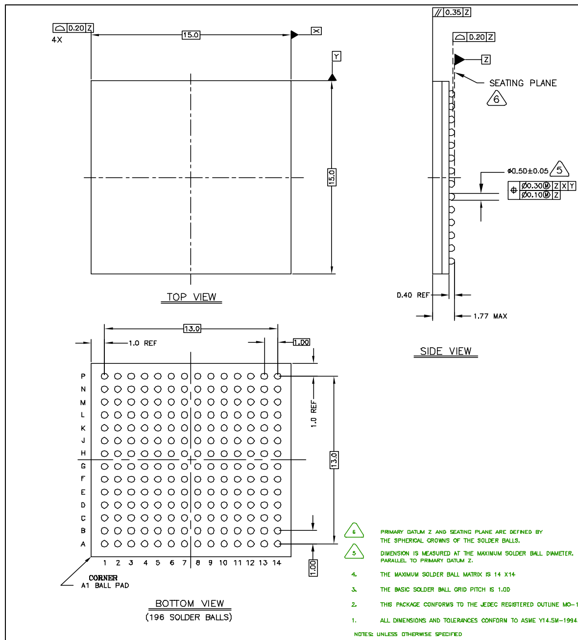
Figure 42: 196-pin FBGA Package Drawing
