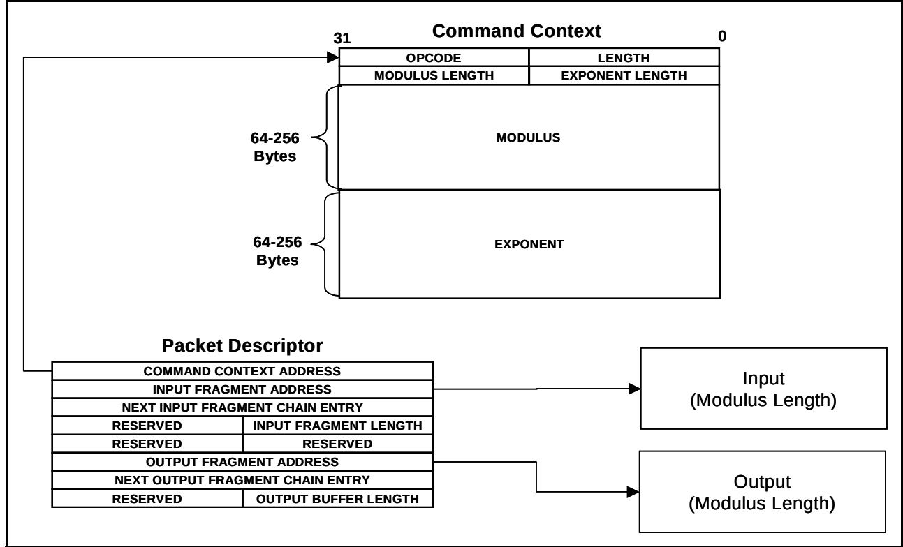
Figure 27: RSA Public Key
