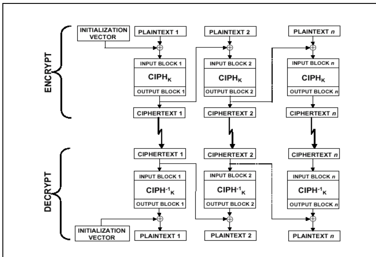
Figure 7: CBC Mode
