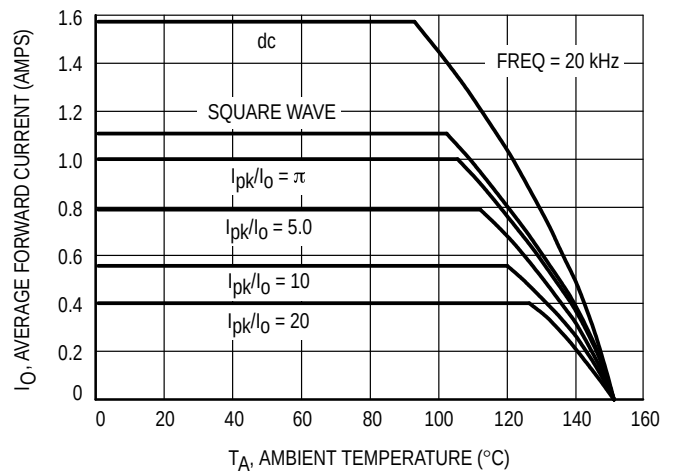
Figure 20. Current Derating
