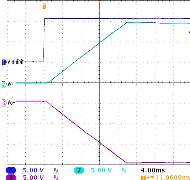
MTR2815D START-UP INTO NO LOAD, 1500 µF CAP LOAD EACH
