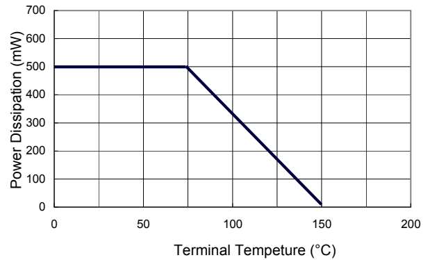
FIG 4 Power Dissipation Curve
