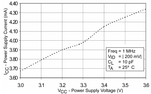
FIGURE 20. Power Supply Current vs. Power Supply Voltage
