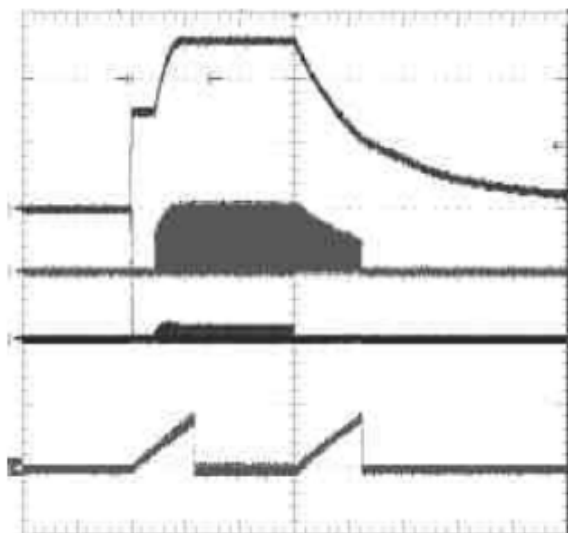
Power on and off under light load
