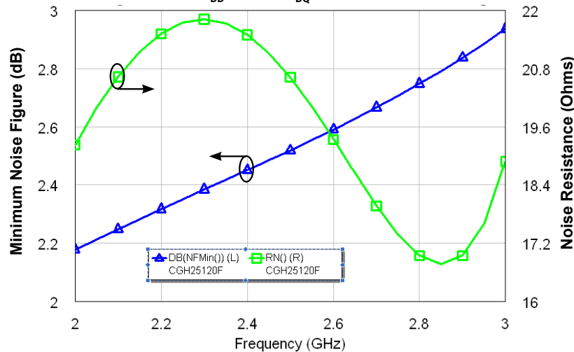
Simulated Minimum Noise Figure and Noise Resistance vs Frequency of the CGH25120F
