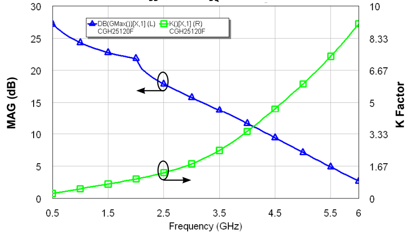
Simulated Maximum Available Gain and K Factor of the CGH25120F
