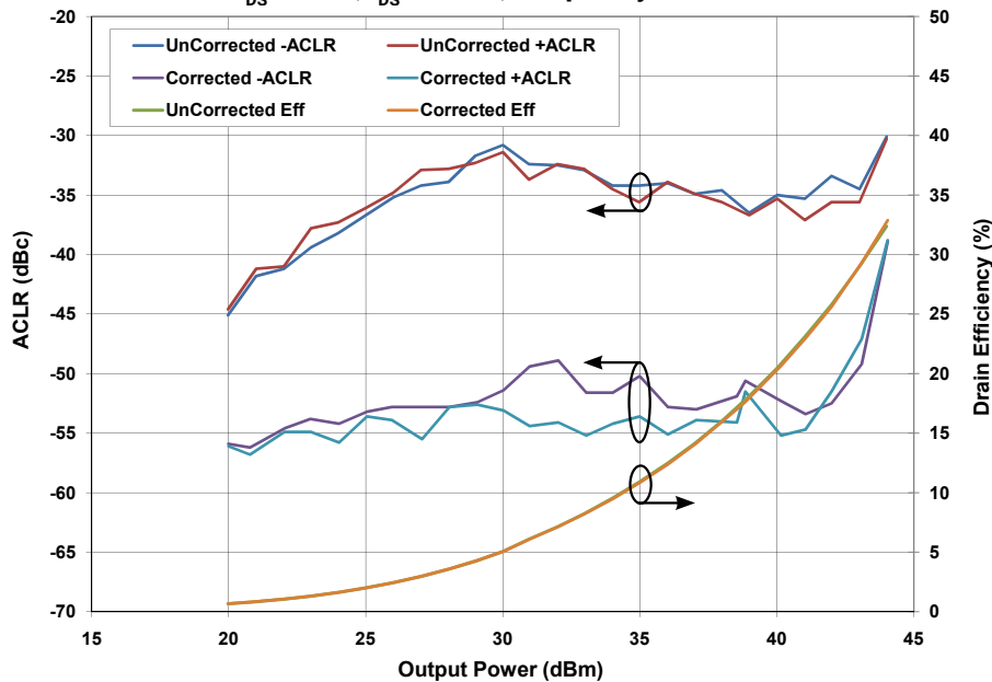
WiMAX Characteristics with and without DPD Correction ACLR and Drain Efficiency vs Output Power measured in CGH25120F-AMP Amplifier Circuit. V_{DS} = 28\text{ V}, I_{DS} = 0.5\text{ A}, \text{Frequency} = 2.5\text{ GHz}
