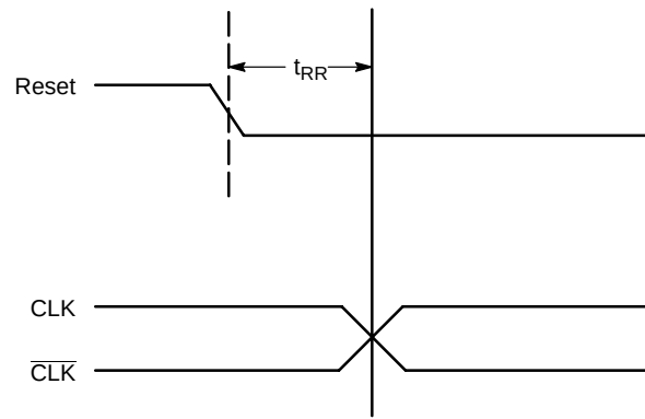
Figure 3. Reset Recovery
