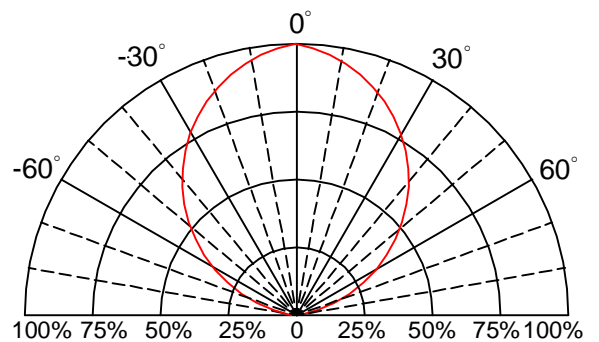
Fig.6 Directive Radiation
