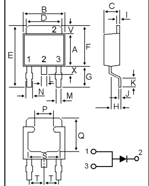
TO-252AA (DPAK)
