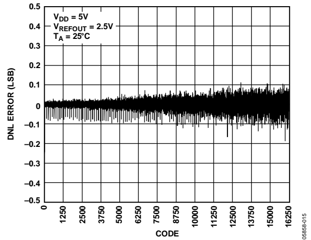
Figure 14. DNL—AD5643R-5
