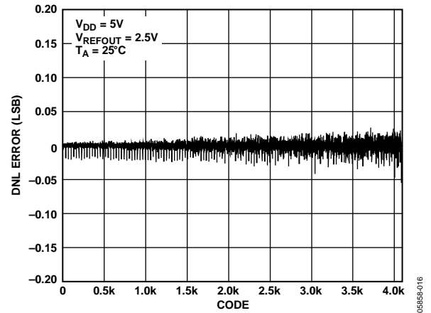
Figure 15. DNL—AD5623R-5
