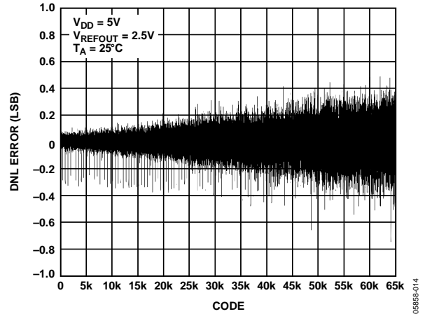
Figure 13. DNL—AD5663R-5
