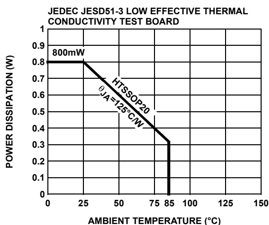
FIGURE 16. PACKAGE POWER DISSIPATION vs AMBIENT TEMPERATURE
