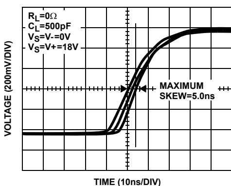
FIGURE 13. SKEW
