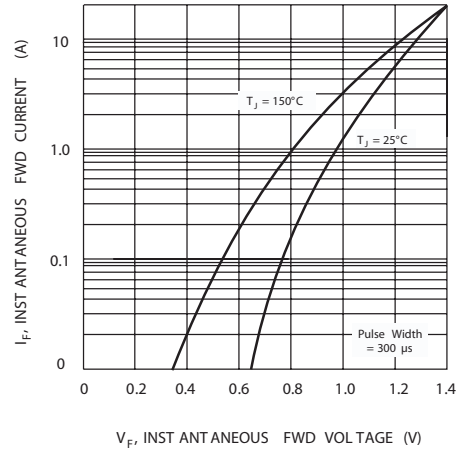
V F , INSTANTANEOUS FWD VOLTAGE (V) Fig. 2 Typical Fwd Characteristics
