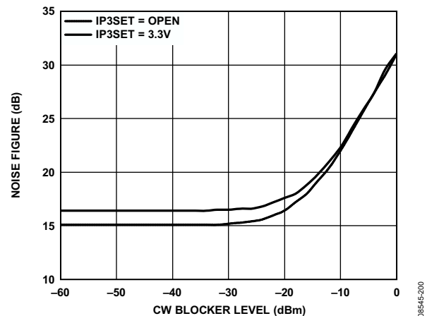
Figure 19. SSB Noise Figure vs. 5 MHz Offset Blocker Level, LO Frequency = 2105 MHz, RF Frequency = 1965 MHz
