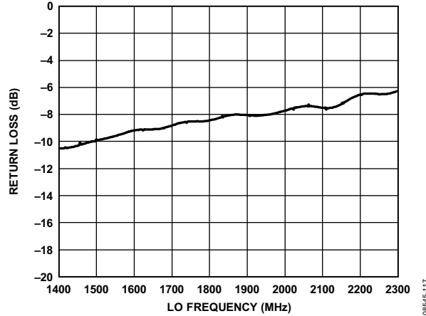
Figure 17. LO Input Return Loss vs. LO Frequency (Including TC1-13 Balun)
