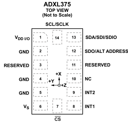
Figure 3. Pin Configuration
