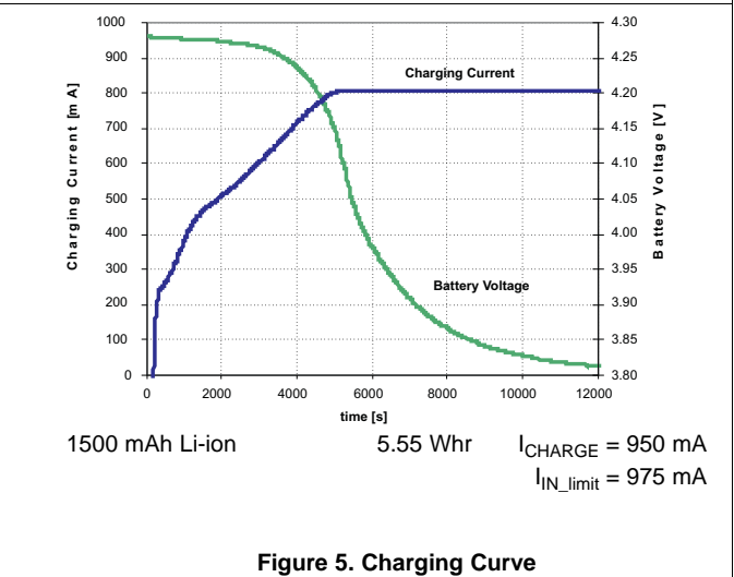
Figure 5. Charging Curve
