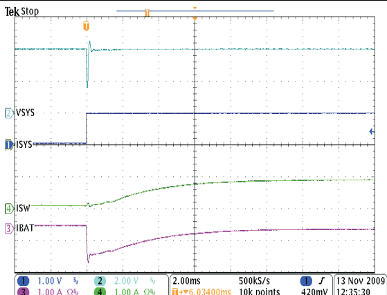
0-A - 1-A Transient on V sys V BUS = 5.5 V V BAT = 4 V V OREG = 4 V I CHARGE = 950 mA I IN_limit = 975 mA
