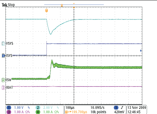
0-A - 1-A Transient on V sys V BUS = 5.5 V No Battery V OREG = 4 V I CHARGE = 950 mA I IN_limit = 975 mA
