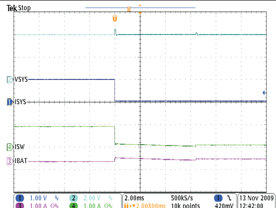
0-A - 1-A Transient on V sys V BUS = 5.5 V V BAT = 4 V V OREG = 4 V I CHARGE = 950 mA I IN_limit = 975 mA
