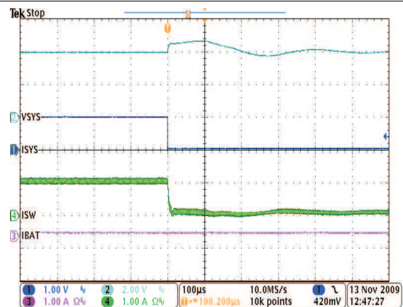
0-A - 1-A Transient on V sys V BUS = 5.5 V No Battery V OREG = 4 V I CHARGE = 950 mA I IN_limit = 975 mA
