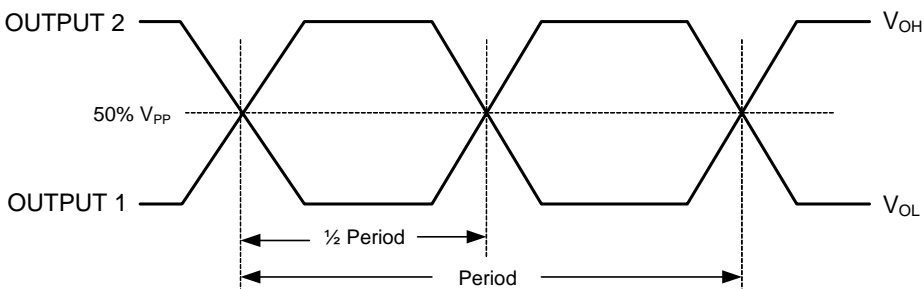
Oscillator Symmetry
