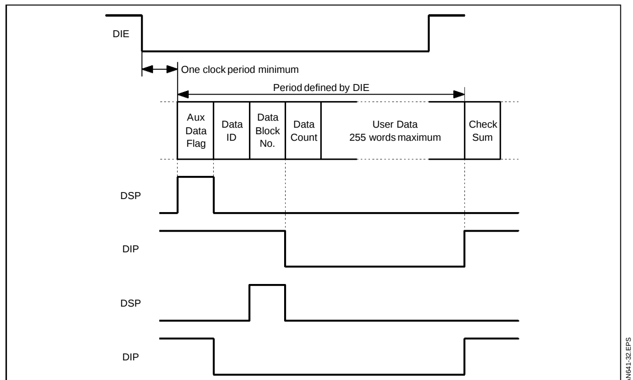
Figure 31 : Timing Requirements for DIP and DSP
