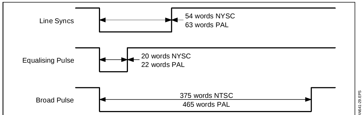
Figure 28 : DIE Pulse Durations
