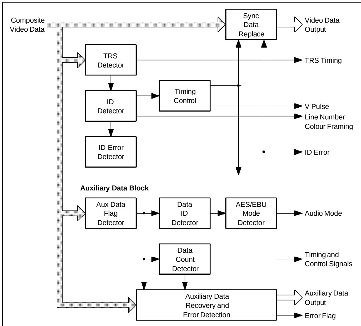
Figure 40 : The receiver Co-Processor
