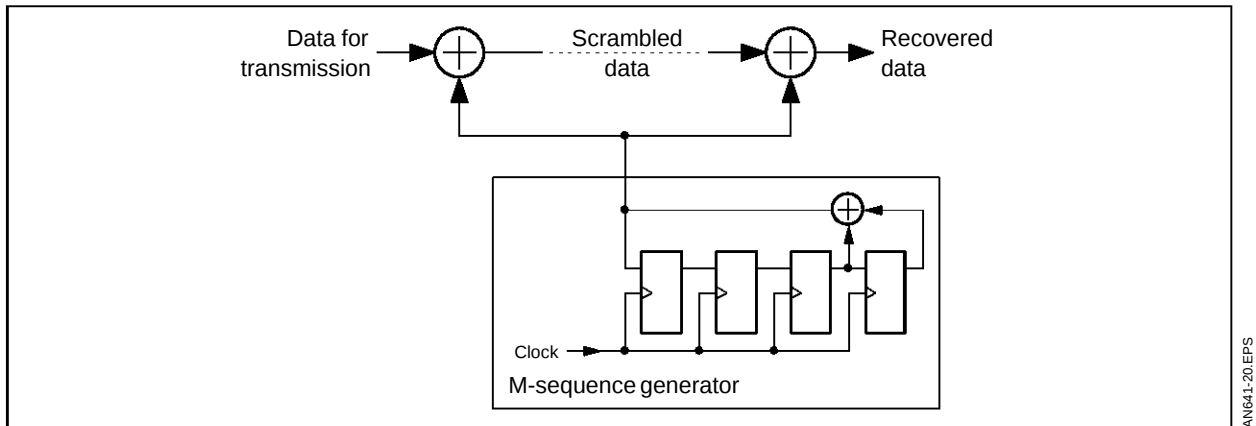
Figure 20 : Self-synchronising Scrambler
