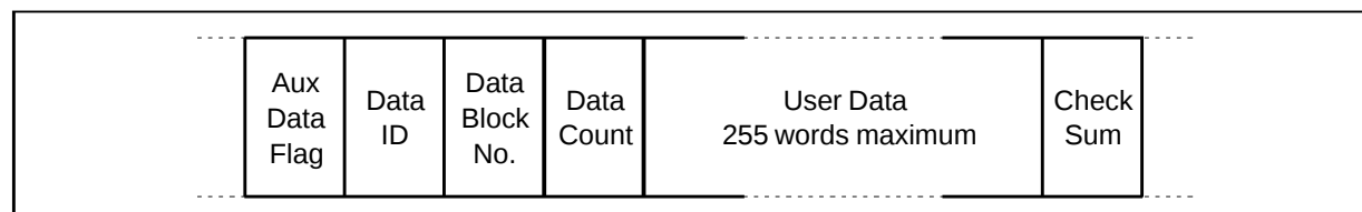
Figure 25 : Auxiliary Data Format
