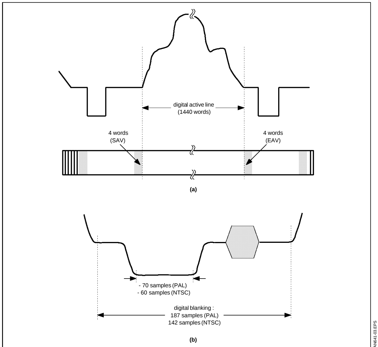
Figure 3 : Horizontal Timing relationships for : (a) component and (b) Composite Digital Video Signals
