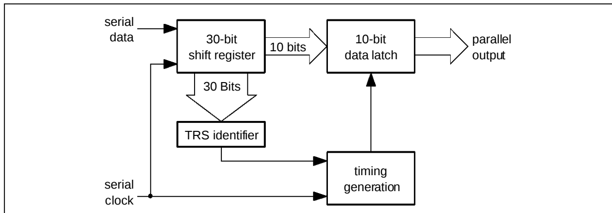
Figure 39 : Serial-to-parallel Conversion
