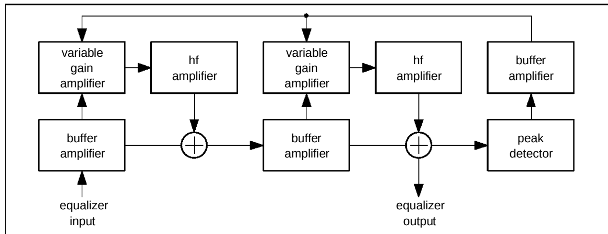
Figure 35 : Cable Equalizer
