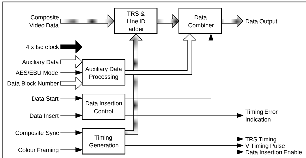
Figure 27 : Transmitter Co-processor Block Diagram
