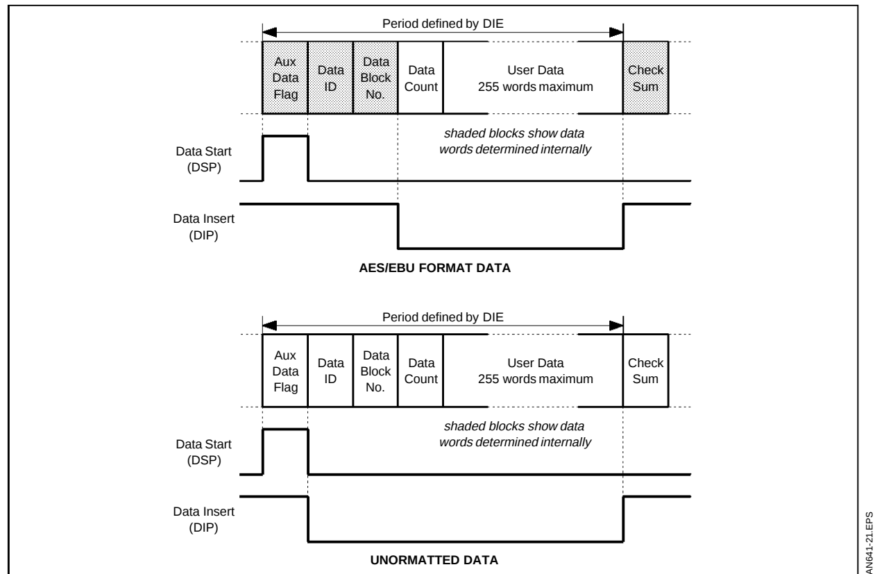
Figure 31 : Timing Requirements for DIP and DSP
