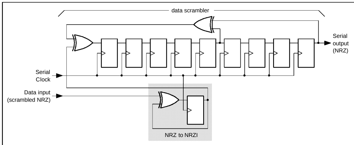
Figure 38 : Data De-Scrambling
