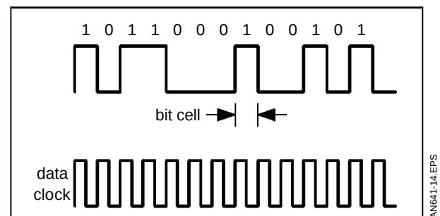
Figure 14 : NRZ Code
