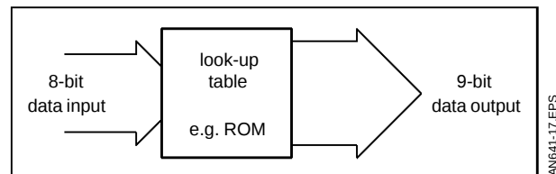
Figure 17 : Example of 8/9 Code Implementation
