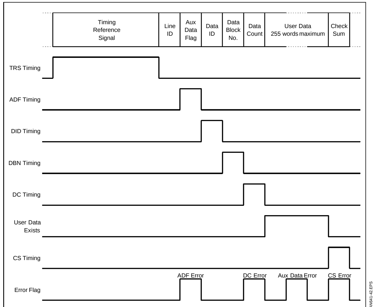
Figure 41 : Timing Control Signals
