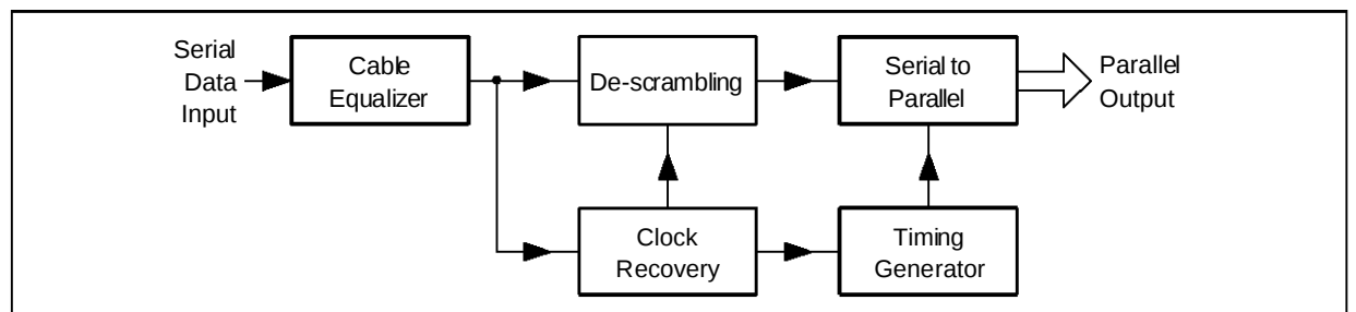
Figure 33 : Serial Decoder Overview
