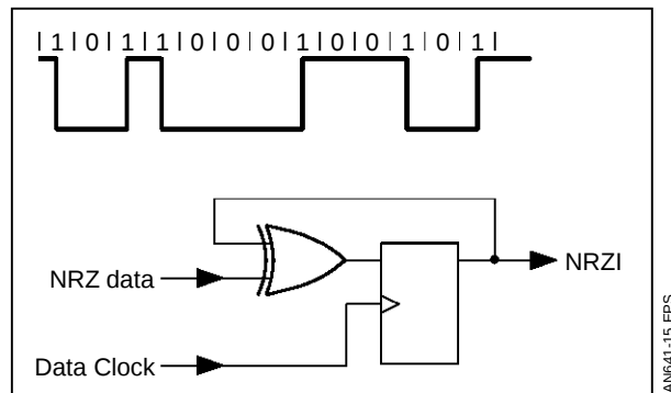
Figure 15 : NRZI code
