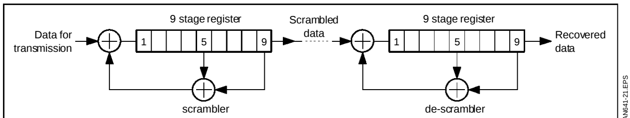
Figure 20 : Self-synchronising Scrambler
