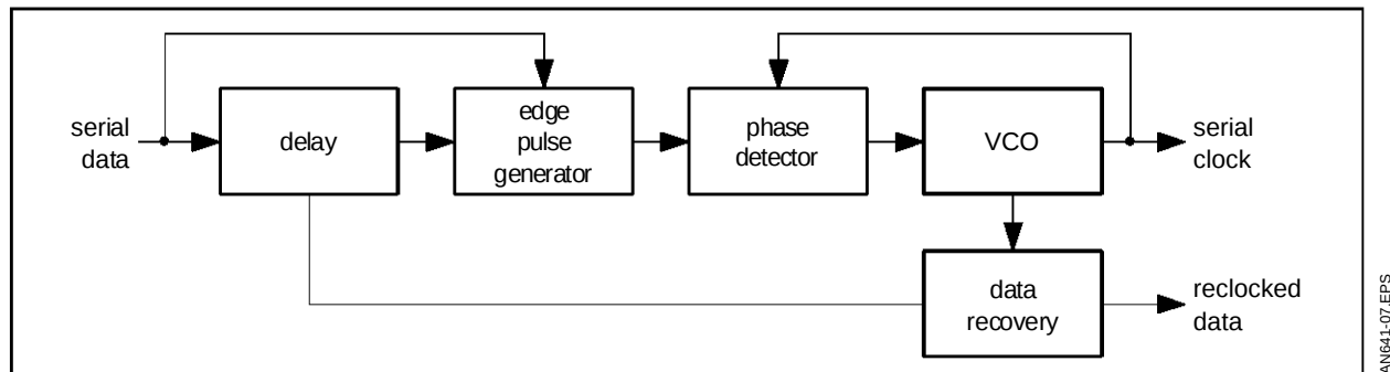
Figure 7 : Obtaining the Clock Information
