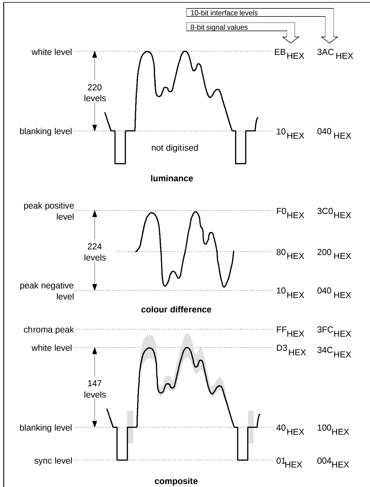
Figure 5 : Range of data Values for Digital Video Signals
