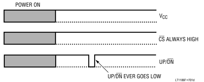
Figure 1d. Pulse Mode Setup (Increment/Decrement)
