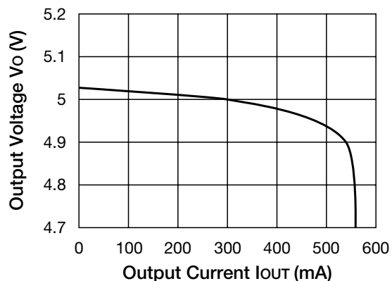
Load Regulation( V_o=5.0\text{V} )
