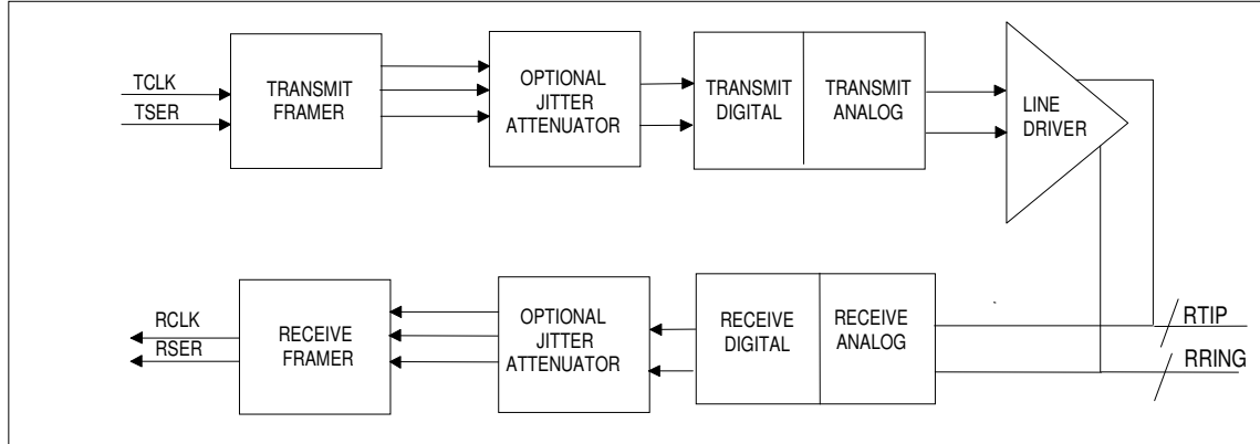
Figure 8-22. Analog Loopback
