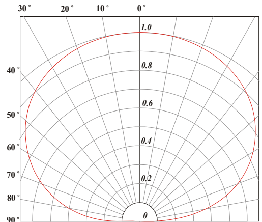
Radiation Pattern
